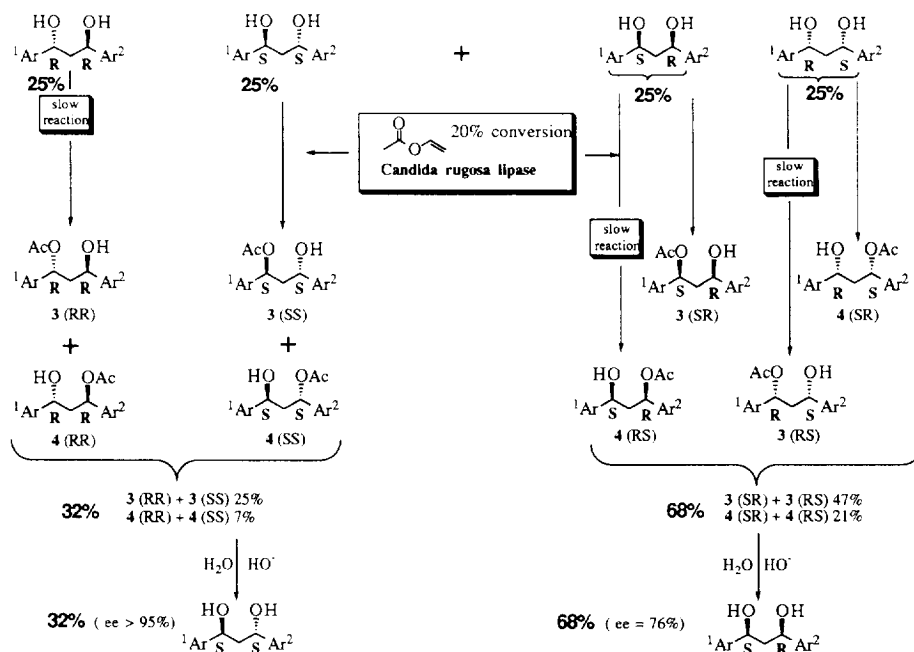
Scheme 2 : Lipase catalysed transesterification of the diastereomeric mixture of the 1,3-diols 2 (Ar 1 and Ar 2 represent the p -methoxyphenyl and the p -nitrophenyl groups respectively).
