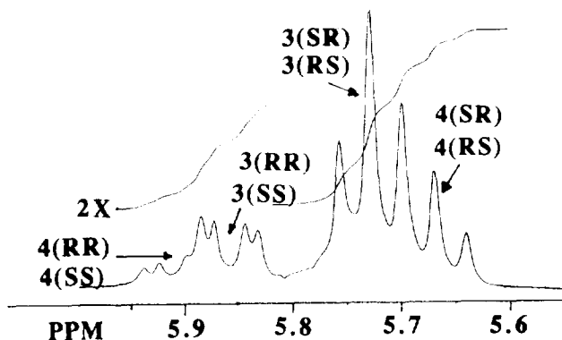
Figure II : ^1\text{H} NMR spectrum (proton near the acetoxy group only shown, solvent : \text{CDCl}_3 ) of the monoacetates obtained with the enzymatic transesterification of the diastereomeric mixture of the 3- p -methoxyphenyl,1- p -nitrophenylpropan-3-ol (2X on the spectrum means the integration of the signals between 5.8 and 6.0 ppm was multiplied by a factor two).
