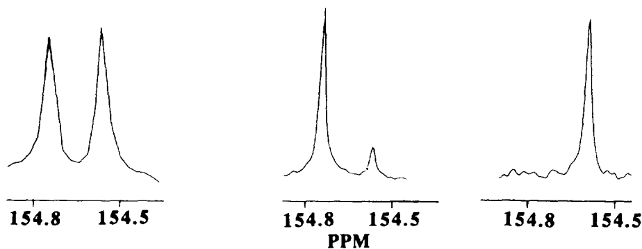
Figure 1 : 13 C NMR spectra (carbonyl groups only, solvent : pyridine- d 5 ) of the di(-)-menthylcarbonates of the (1 R ,3 R /1 S ,3 S )-1,3-diphenyl-1,3-diol 1 . Left : from the racemic diol, middle : from the remaining alcohol (mainly 1 R ,3 R ), right : from the hydrolysis of the acetate produced in the enzymatic resolution, (nearly pure 1 S ,3 S ).
