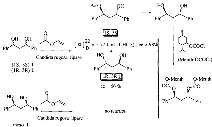
Scheme 1 : Lipase catalyzed transesterification of the 1,3-diphenylpropane-1,3-diols 1 .
